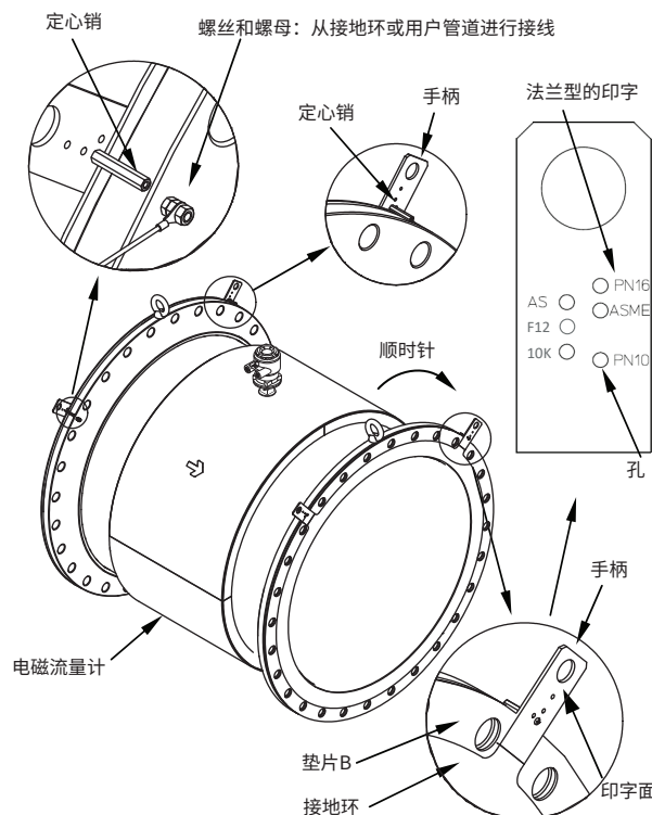
图3.3.4 带接地环GR1的安装步骤(口径不超过1000 mm (40 in.))
